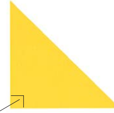
right-angled triangle
